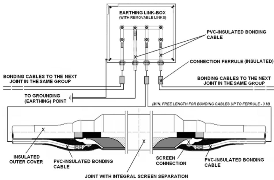
Figure 1 - Principle connection scheme for bonding cables at the transition joints.
